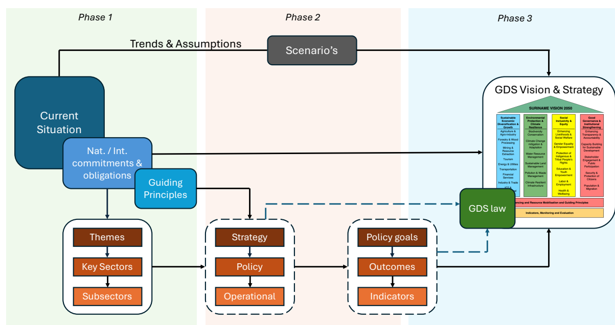
Figure 12: GDS Methodology
